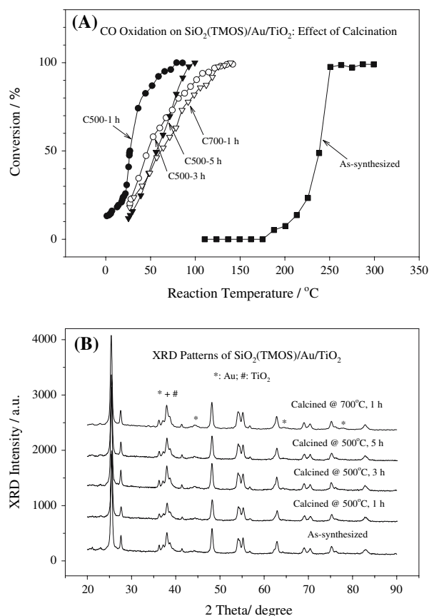
Figure 3. CO light-off curves (figure 3A) and XRD patterns (figure 3B) of as-synthesized \text{SiO}_2(\text{TMOS})/\text{Au}/\text{TiO}_2 and those further calcined in \text{O}_2 -He at 500 °C for 1–5 h or at 700 °C for 1 h.
