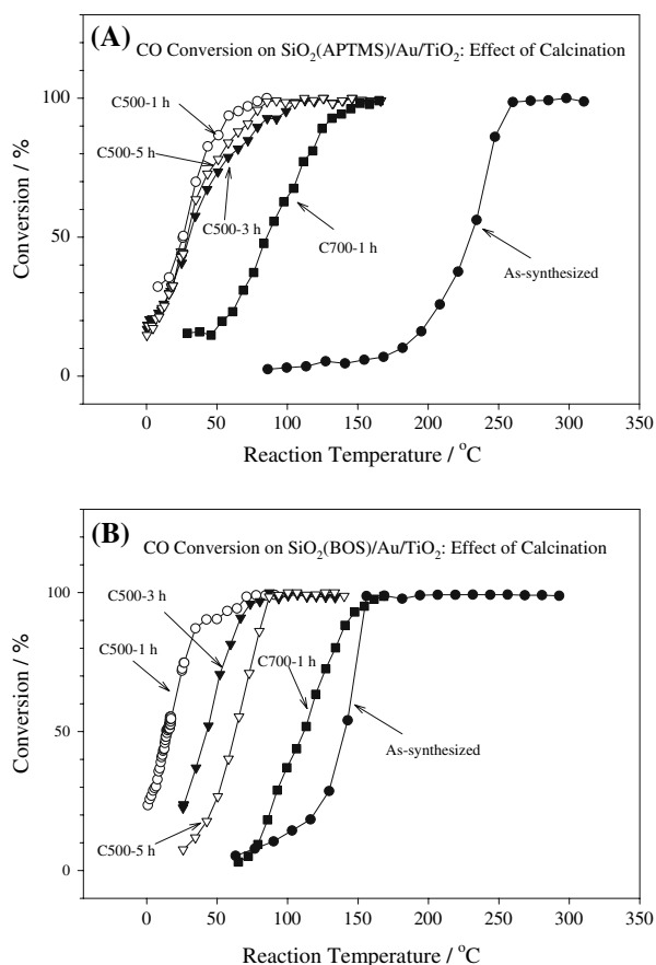
Figure 6. Panel A: CO light-off curves of as-synthesized \text{SiO}_2(\text{APTMS})/\text{Au}/\text{TiO}_2 and those further calcined in \text{O}_2 -He at 500 °C for 1–5 h or at 700 °C for 1 h. Panel B: CO light-off curves of as-synthesized \text{SiO}_2(\text{BOS})/\text{Au}/\text{TiO}_2 and those further calcined in \text{O}_2 -He at 500 °C for 1–5 h or at 700 °C for 1 h.
