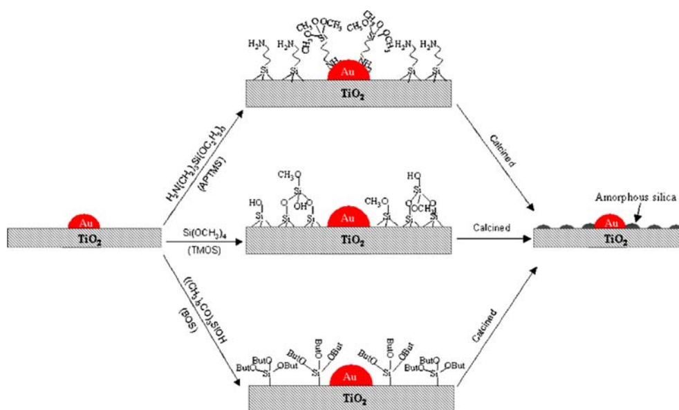
Figure 1. Proposed scheme for the synthesis of \text{SiO}_2 -decorated \text{Au/TiO}_2 . Pre-formed \text{Au/TiO}_2 was treated in tetramethyl orthosilane (TMOS, \text{Si}(\text{OCH}_3)_4 ), (3-aminopropyl)trimethoxysilane (APTMS, \text{H}_2\text{N}(\text{CH}_2)_3\text{Si}(\text{OC}_2\text{H}_5)_3 ), or tris( tert -butoxy)silanol (BOS, ((\text{CH}_3)_3\text{CO})_3\text{SiOH} ) solution, followed by calcination.
