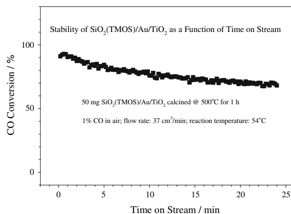
Figure 7. CO conversion on 500 °C-calcined \text{SiO}_2(\text{TMOS})/\text{Au}/\text{TiO}_2 as a function of reaction time.
