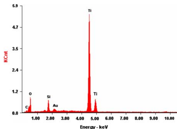
Figure 5. EDAX data of \text{SiO}_2(\text{TMOS})/\text{Au}/\text{TiO}_2 which was calcined in \text{O}_2 -He at 500 °C.
